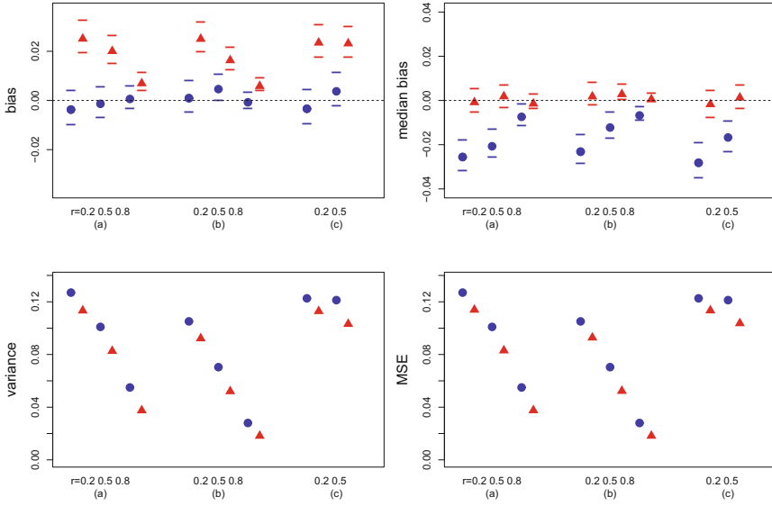
Fig. 4.2 Simulation results of the bias and median bias with confidence intervals as well as variance and MSE of the estimators \hat{\lambda}_1^{block} (red filled triangle) and \hat{\lambda}_1^{pd} (blue filled circle) with F_1 = \dots = F_k , k = 4 and n = 10 with an underlying \log \mathcal{N}(0, 1) distribution and CS (a), AR(1) (b) and MA(1) (c) covariance structures
