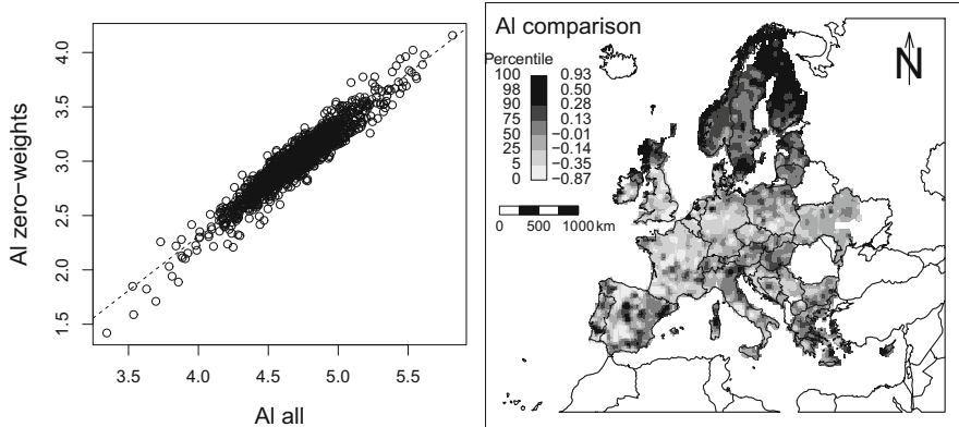
Fig. 10.2 Comparison of the two balances used for mapping AI in Fig. 10.1. Left : scatterplot of the two balances, with main trend indicated by the dashed line ; right : orthogonal deviations from the dashed line are mapped, indicating the difference between both maps in Fig. 10.1
