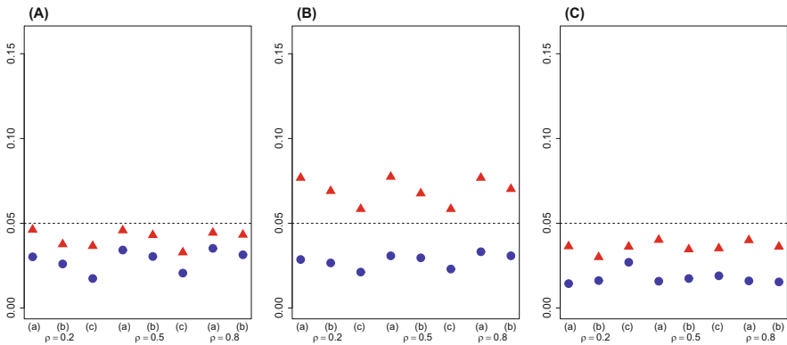
Fig. 4.6 Non-coverage probabilities of normal (A), basic (B), and studentized (C) bootstrap confidence intervals for the estimators \hat{\lambda}_1^{block} (red filled triangle) and \hat{\lambda}_1^{pd} (blue filled circle) with F_1 = \dots = F_k , an underlying \log \mathcal{N}(0, 1) distribution, \alpha = 0.05 , k = 4 , n = 10 and underlying CS (a), AR(1) (b) and MA(1) (c) covariance structures
