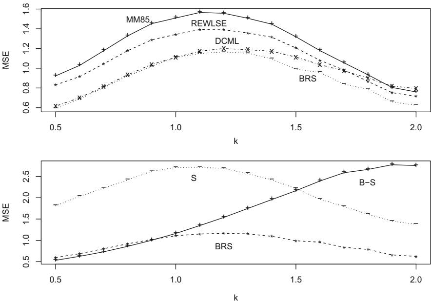
Fig. 6.1 MSEs of regression estimators as function of outlier size k for normal \mathbf{x} , p = 10 , n = 50 and \varepsilon = 0.1 . Note that the y -axis of the upper panel is zoomed in from the y -axis of the lower panel
