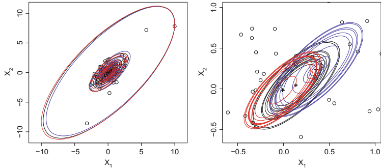
Fig. 18.6 t -distribution: Mahalanobis distances represented by co-axial ellipses centered at the mean \bar{X} ( black ), at the trimmed L_{n1} -estimator ( blue ) and at the L_{n2} -estimator ( red ). All simulated bivariate data with the every tenth contour are illustrated on the left , detail of the center with the first ten contours is on the right
