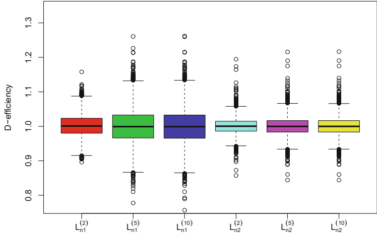
Fig. 18.5 t -distribution: box-plots of the 5000 estimated values of D-efficiency for the L_{n1}^{(2)} , L_{n1}^{(5)} , L_{n1}^{(10)} , L_{n2}^{(2)} , L_{n2}^{(5)} , L_{n2}^{(10)}
