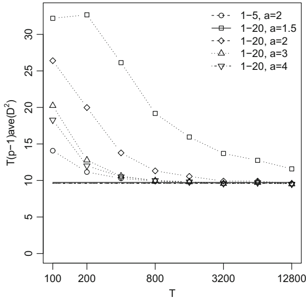
Fig. 25.2 The averages of T(p-1)\hat{D}^2 over 10,000 repetitions of the observed time series with length T from model (ii) for the different estimates. The horizontal lines give the expected values of the limiting distributions of T(p-1)\hat{D}^2
