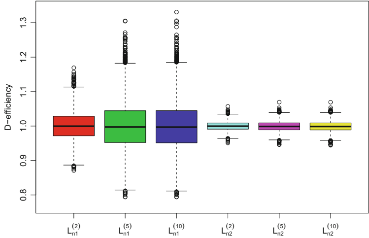
Fig. 18.2 Normal distribution: box-plots of the 5000 estimated values of D-efficiency for the L_{n1}^{(2)} , L_{n1}^{(5)} , L_{n1}^{(10)} , L_{n2}^{(2)} , L_{n2}^{(5)} , L_{n2}^{(10)}
