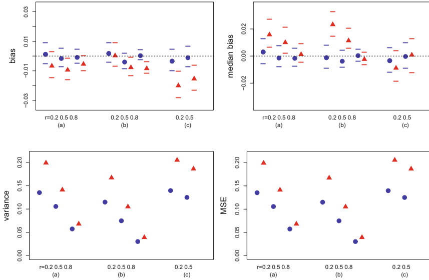
Fig. 4.3 Simulation results of the bias and median bias with confidence intervals as well as variance and MSE of the estimators \hat{\lambda}_1^{block} (red filled triangle) and \hat{\lambda}_1^{pd} (blue filled circle) with F_j = F(x - \alpha_j) , \forall j , k = 4 and n = 10 with an underlying \mathcal{N}(0, 1) distribution and CS (a), AR(1) (b) and MA(1) (c) covariance structures
