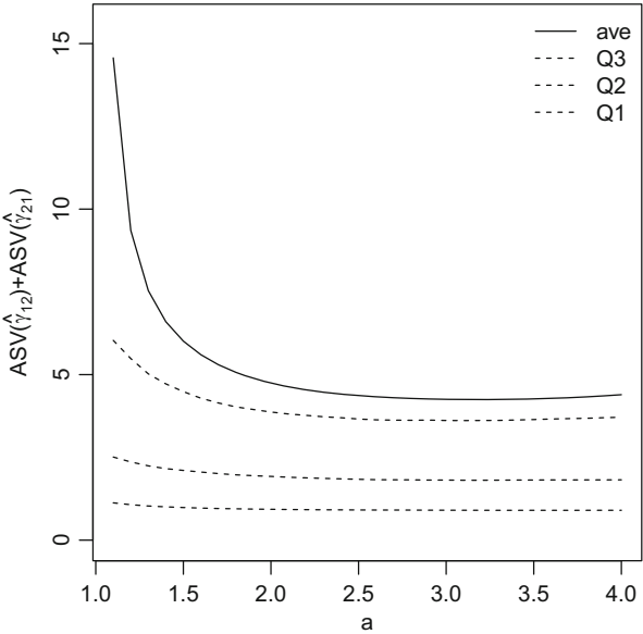
Fig. 25.3 The averages and the quartiles of the sum ASV(\hat{y}_{12}) + ASV(\hat{y}_{21}) from 10,000 pairs of source time series, that were generated as described in Sect. 25.4.2
