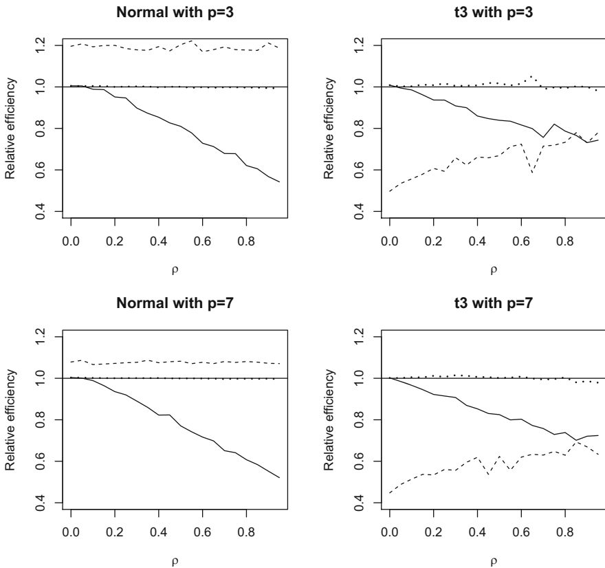
Fig. 13.1 Efficiency relative to the transformation–retransformation L_1 method with estimated \rho . Equal \rho case. Basic L_1 is the full line (—), mixed model is the dashed line (---), transformed L_1 with true \rho is the dotted line (···)
