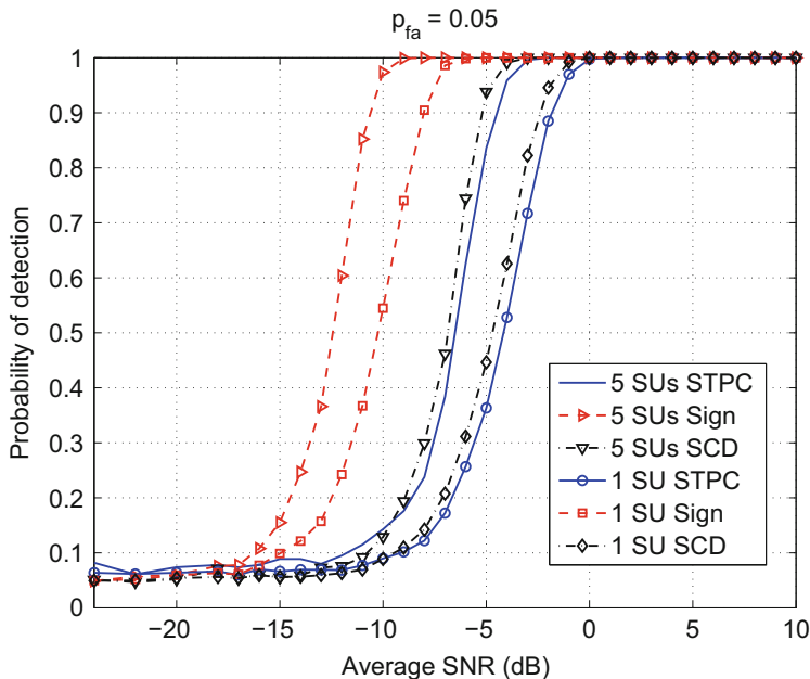
Fig. 27.5 Probability of detection vs. SNR (dB) in a contaminated additive Gaussian noise channel for 1 and 5 secondary users. Additive noise has a contaminated Gaussian distribution 0.95N_C(0, \sigma^2) + 0.05N_C(0, 100\sigma^2) . SNR is defined with respect to \sigma^2 . The signal is an OFDM signal (DVB-T). The spatial sign cyclic correlation based detector is more robust against heavy-tailed non-Gaussian noise than the other considered detectors
