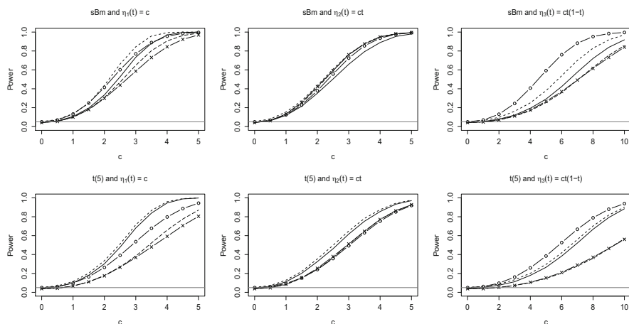
Fig. 20.2 Plots of the asymptotic powers of the tests based on T_S (—), T_{SR} (---), T_1 (···), T_2 (—×—) and T_3 (—○—) for the sBm and the t(5) distributions under shrinking location shifts
