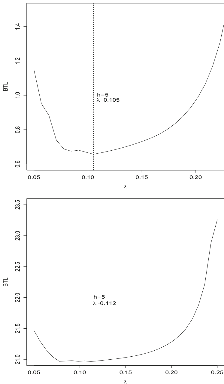
Fig. 14.1 BTL-criterion as a function of tuning parameter \lambda for the original data ( top ) and the contaminated data ( bottom ). The parameter h gives the number of non-zero regression vectors \beta_j including the intercept
